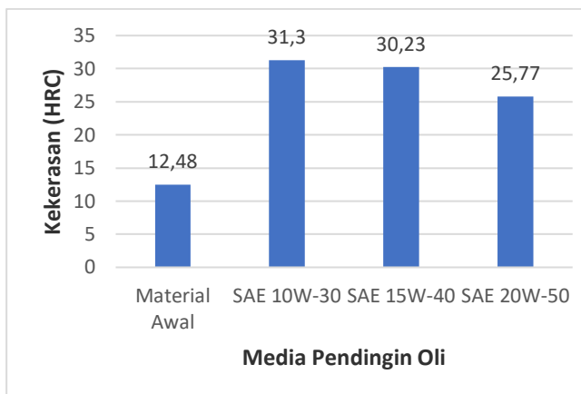
Gambar 2. Grafik nilai kekerasan rata-rata holding time 30 menit
