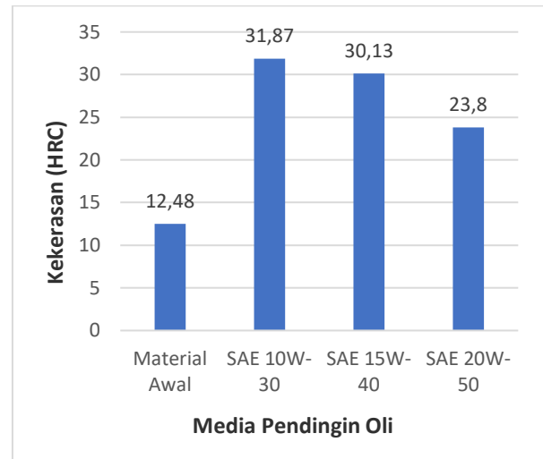
Gambar 3. Grafik nilai kekerasan rata-rata holding time 50 menit
